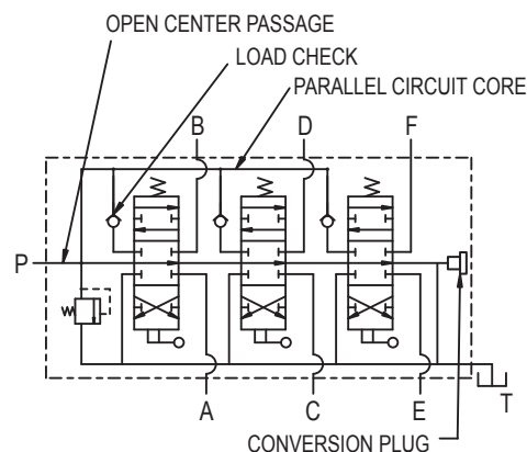
The above drawing shows a symbol for a Three-Spool Valve Model Number RD532CCCAA5A4B1
